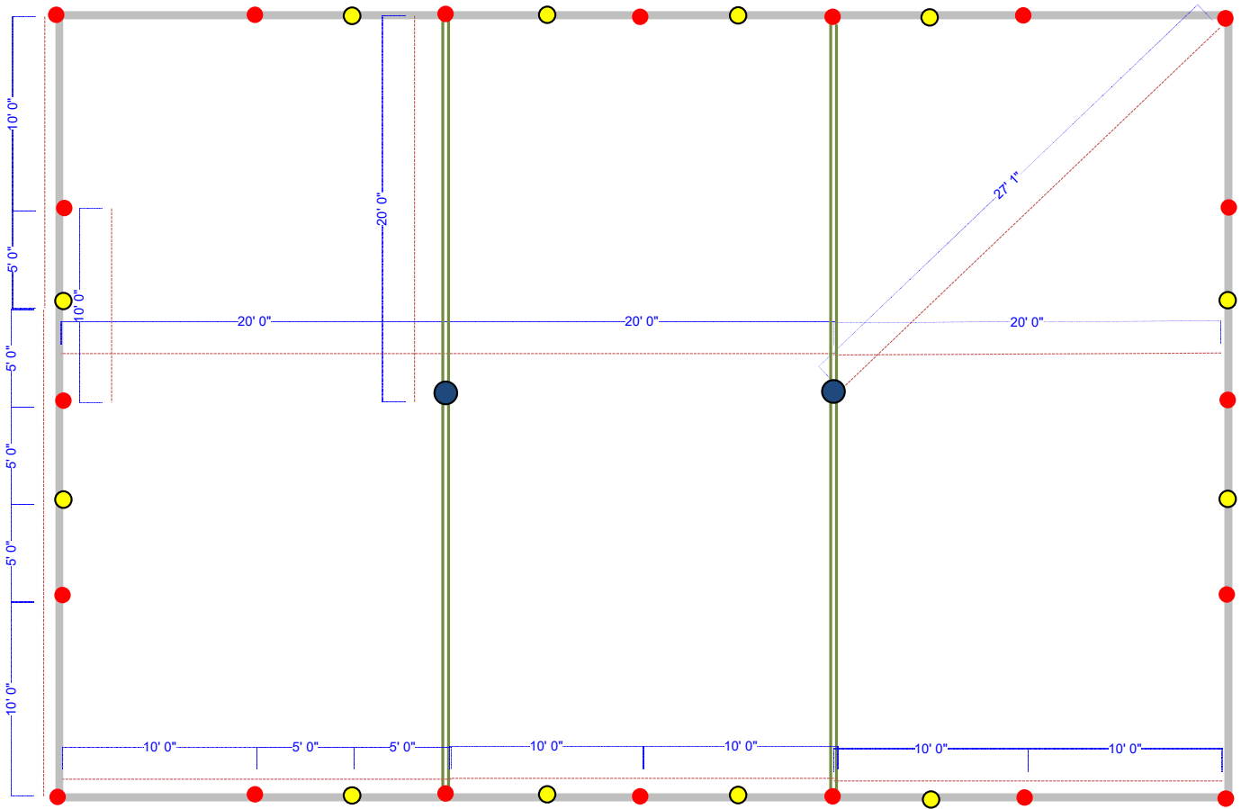
40' x 60' Pole Tent Standard & Wind - Pole Placements
